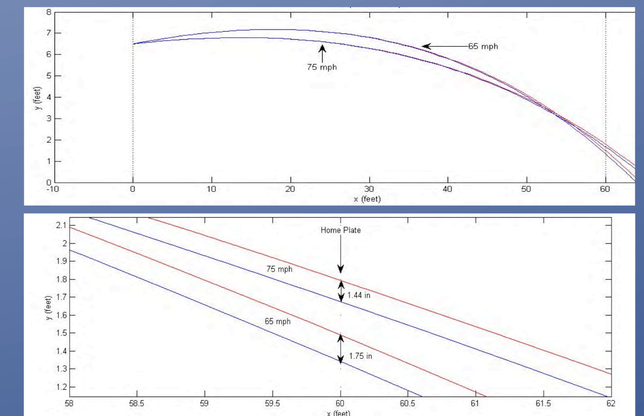
Figure 4.5: Comparing the path of the 65 and 75 mph curveballs. The red line represents the flat-seam ball, and the raised-seam ball is in blue. In order to cross the plate at around the same height as the 75 mph pitch, the 65 mph pitch must have a greater initial launch angle. In the slower pitch, the baseball travels a greater distance for a longer amount of time, resulting in a greater difference in vertical deflection between the raised and flat-seam baseballs.
