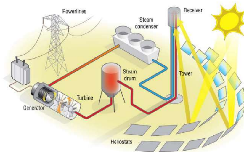
Figure 1.1: Solar power tower diagram. The mirrors focus sunlight to the central tower which houses thermal pipes containing the liquid salt solution. The Ivanpah Solar Power Facility follows this design [4].
