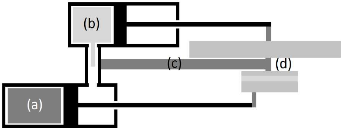
Figure 3.2: Simplified diagram of the Stirling engine used. Notice the oscillatory alignment of the pistons is such that they have a phase difference of \frac{\pi}{2} . (a) Hot piston (b) cold piston (c) brace to hold engine together (d) flywheels.
