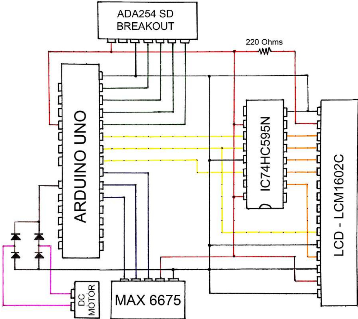
Figure 3.4: Circuit diagram of electrical components.
