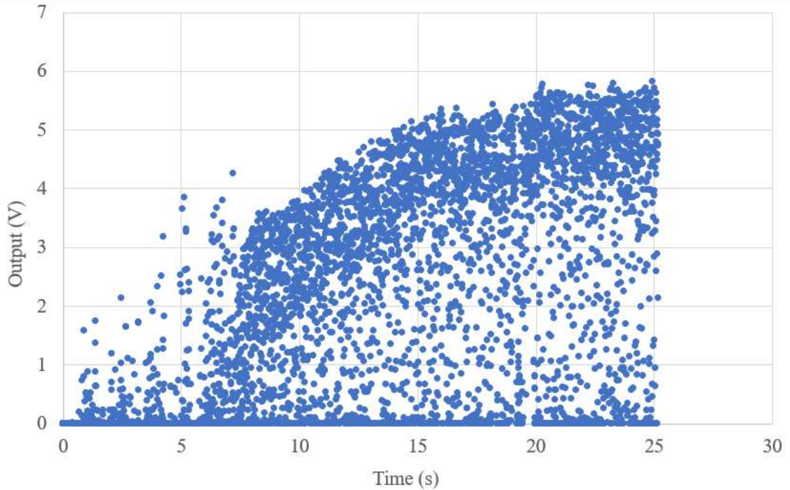
Figure 4.2: Output voltage versus time elapsed during data collection.
