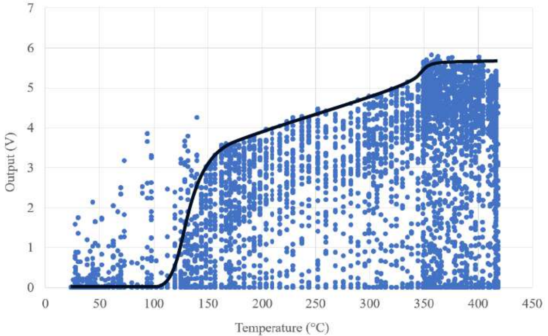
Figure 5.1: Output voltage versus Stirling engine temperature with manual trend line applied.
