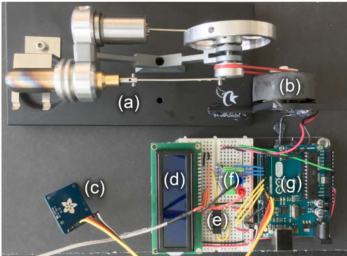
Figure 3.1: Figure of setup. (a) Stirling engine (b) brushless DC motor (c) microSD breakout board (d) LCD screen (e) 8-bit shift register (f) thermocouple module (g) Arduino UNO
