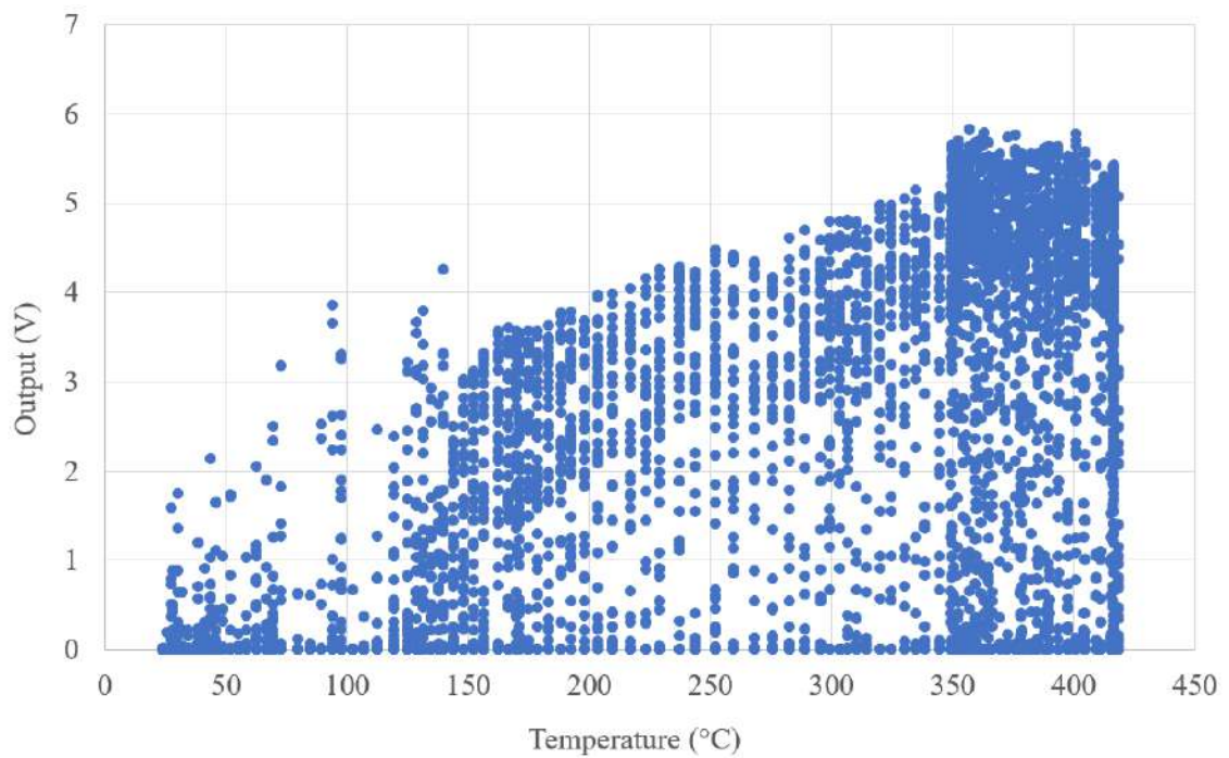
Figure 4.1: Output voltage versus Stirling engine temperature.
